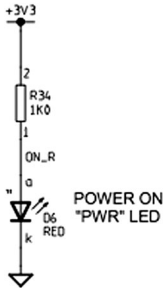
Figure 5-1. Power LED
