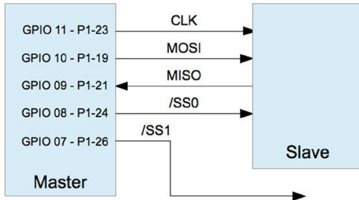
Figure 15-1. SPI interface
