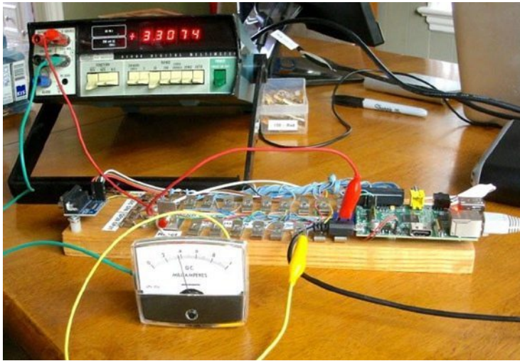
Figure 30-2. A milliamper meter showing 40% deflection
