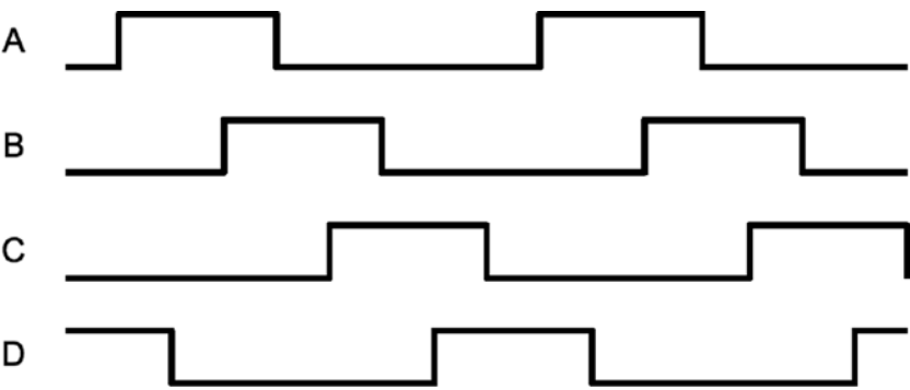
Figure 27-8. Half-step drive
