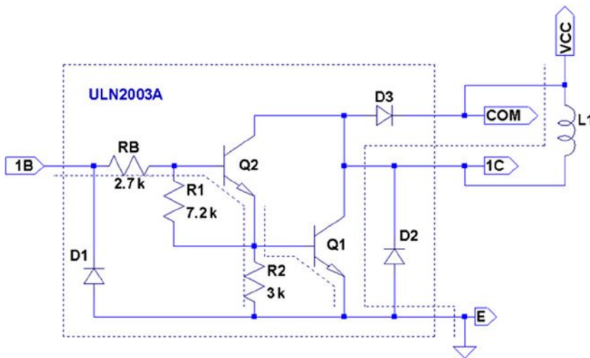
Figure 27-4. ULN2003A driving a winding
