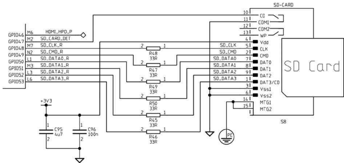
Figure 10-2. SD card circuit
