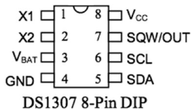
Figure 25-1. DS1307 pinout
