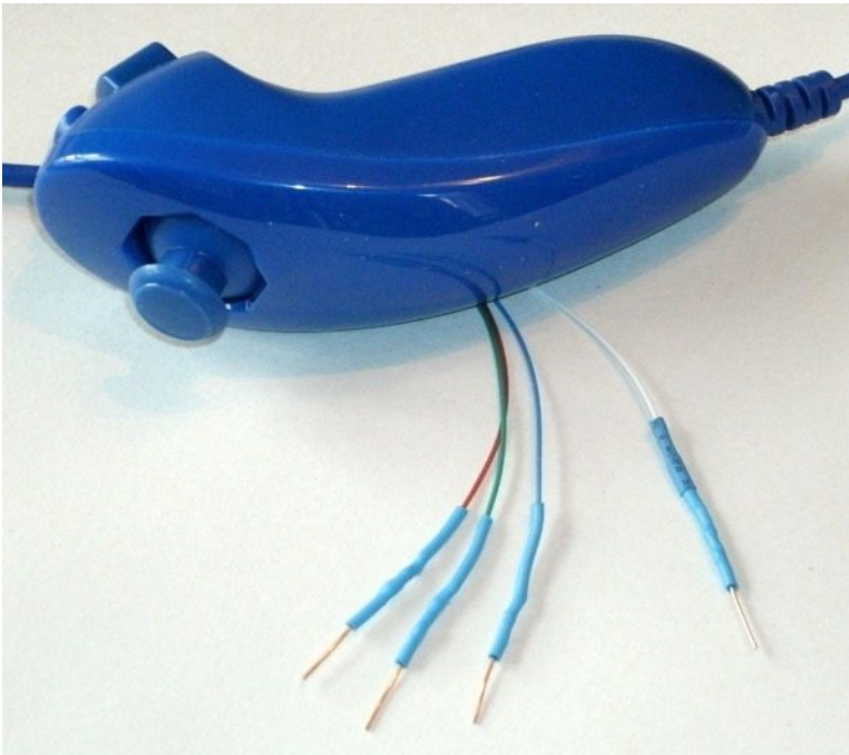
Figure 24-1. Nunchuk with wire ends
