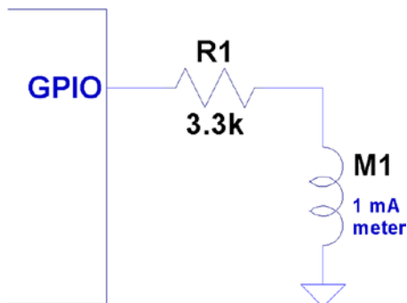
Figure 30-1. PWM-driven meter
