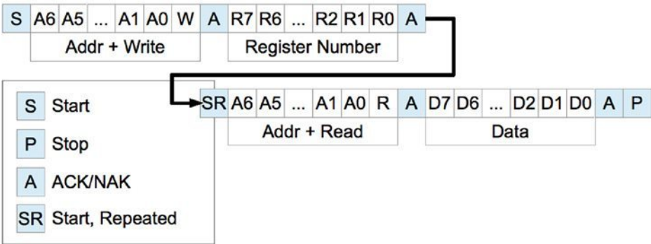
Figure 14-4. Example I2C messages
