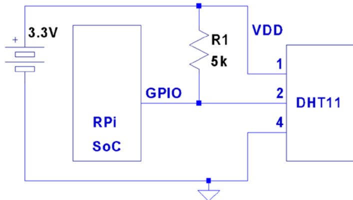
Figure 22-2. DHT11 circuit
