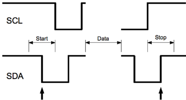
Figure 14-2. I2C start/stop signaling
