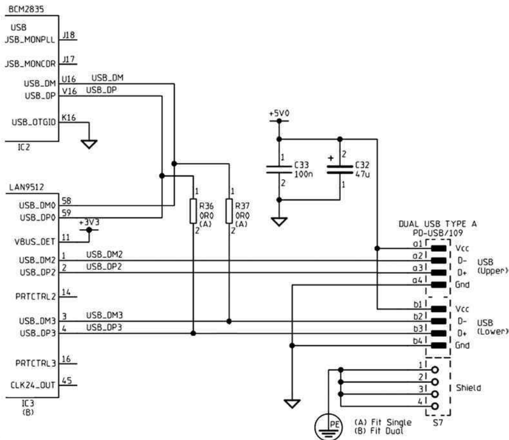
Figure 8-1. USB interface
