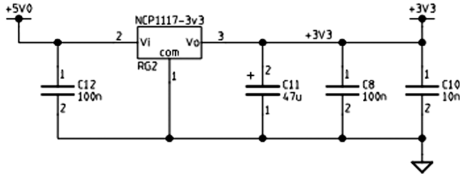
Figure 4-3. 3.3 V power
