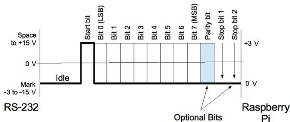
Figure 11-3. Serial signal
