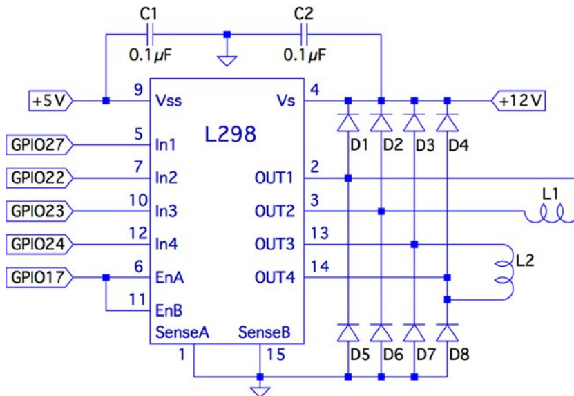
Figure 28-7. L298 schematic
